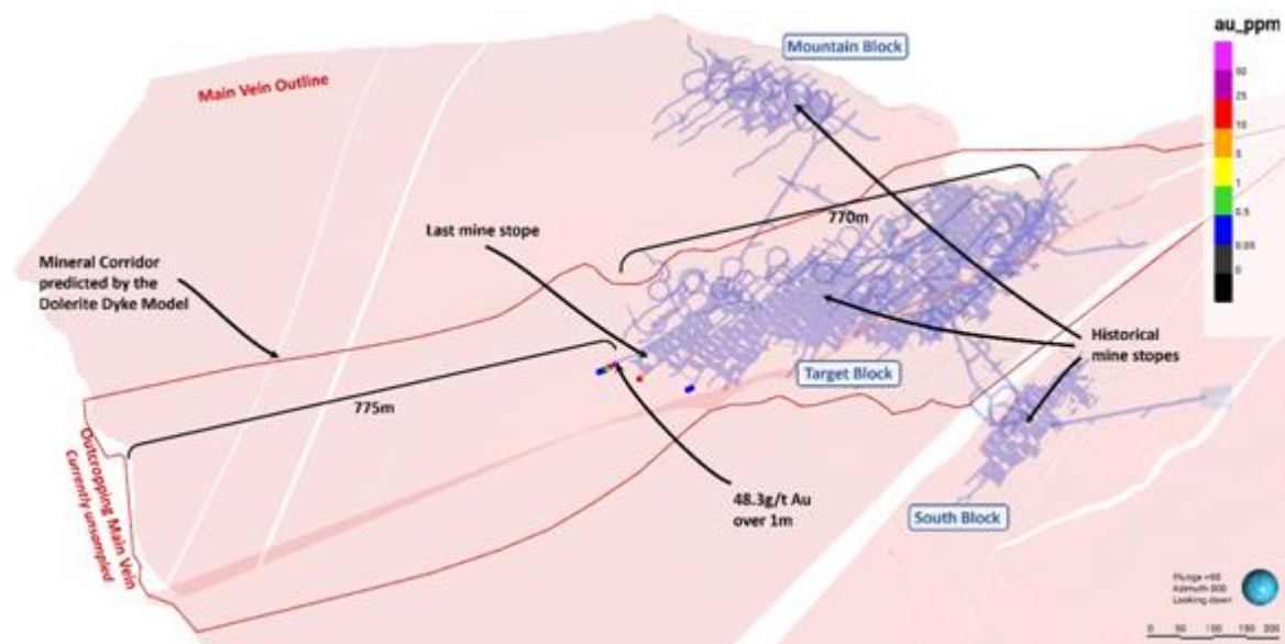
Plan view map with 2023 underground sampling locations and highlighted target block extension potential (Source: www.amaroqminerals.com )
